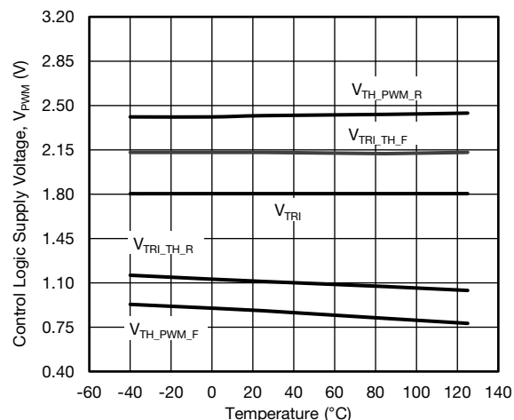
Fig. 13 - PWM Threshold vs. Temperature (SiC632A)
