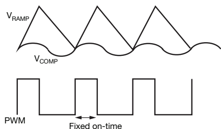
Fig. 5 - Operational Principle
