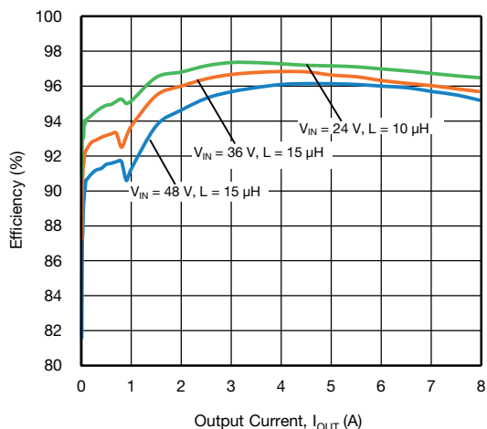
Fig. 17 - SiC477 Efficiency vs. Output Current, V_{OUT} = 12\text{ V}
