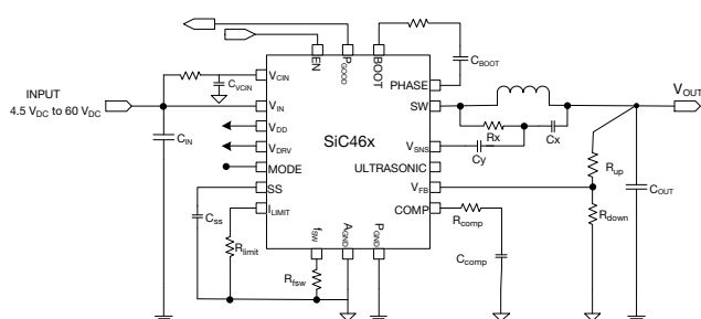
Fig. 1 - Typical Application Circuit for SiC46x
