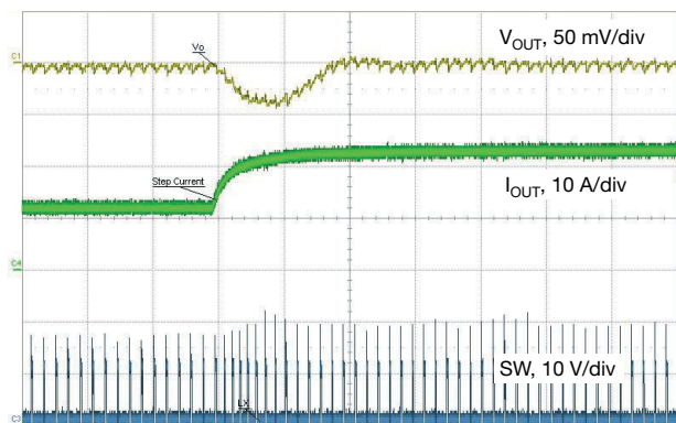
Fig. 30 - Load Step, 12 A to 24 A, 1 A/μs, t = 10 μs/div
