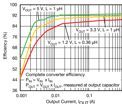
Fig. 13 - Efficiency vs. Output Current ( V_{IN} = 12\text{ V} , f_{sw} = 500\text{ kHz} , Light Load)
