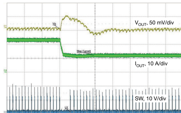
Fig. 33 - Load Release, 24 A to 12 A, 1 A/μs, t = 10 μs/div
