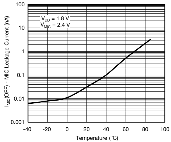
MIC Leakage Current vs. Temperature
