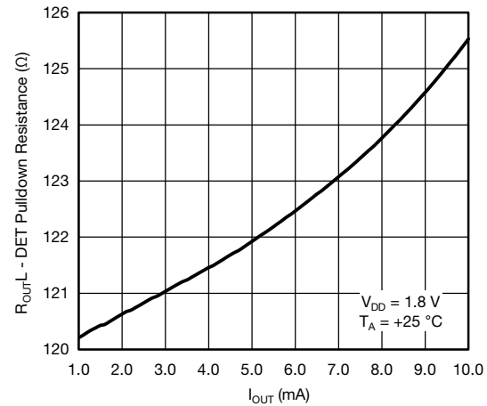
DET Pulldown Resistance vs. I_{\text{OUT}}
