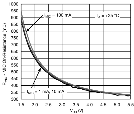
MIC On Resistance vs. V_{\text{DD}}
