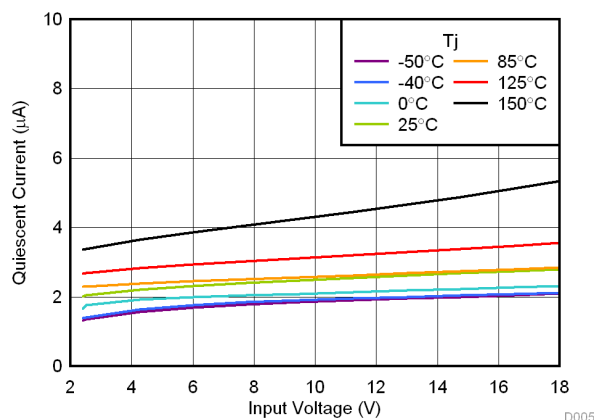
Quiescent Current vs Input Voltage ( V_{OUT} = 1.24 V, I_{OUT} = 0 A)
