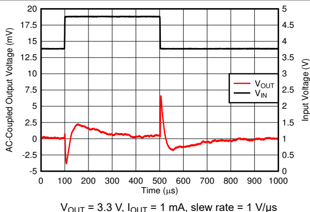
Figure 6-24. Line Transient
