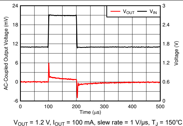
Figure 6-31. Line Transient
