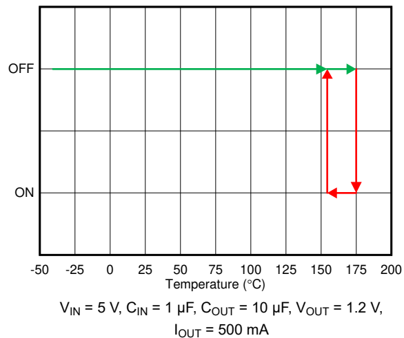
Figure 6-81. Thermal Shutdown Activation
