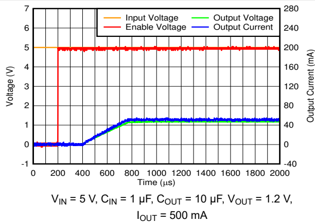
Figure 6-79. Start Up at 25^\circ\text{C}
