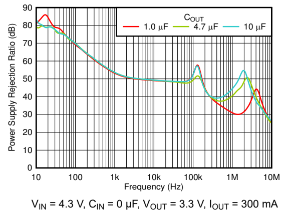
Figure 6-68. PSRR vs Frequency and C_{OUT}
