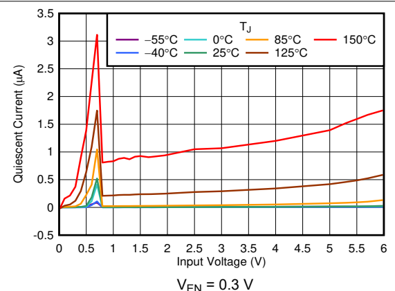
Figure 6-18. I_{SHDN} vs V_{IN}
