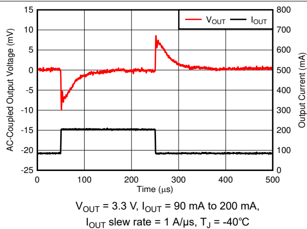
Figure 6-63. Load Transient
