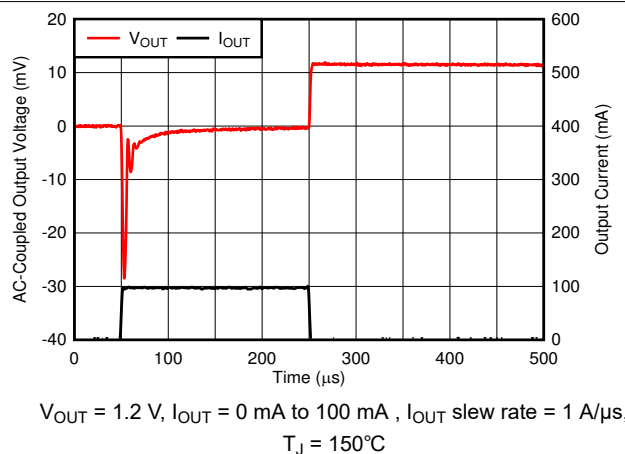
Figure 6-49. Load Transient
