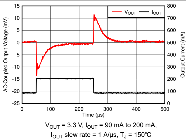
Figure 6-64. Load Transient
