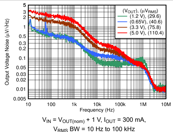
Figure 6-72. Output Noise vs Frequency and V_{OUT}
