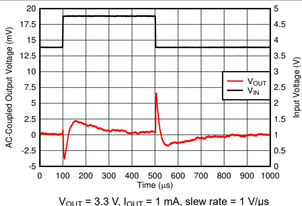
Figure 6-24. Line Transient
