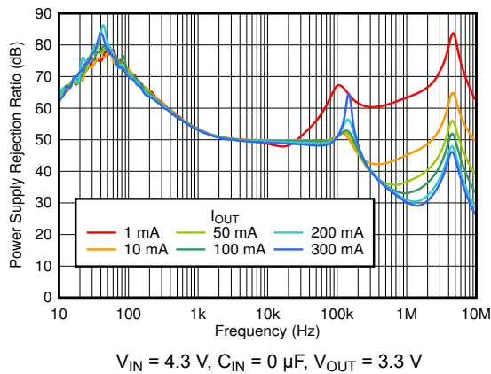
Figure 6-67. PSRR vs Frequency and I_{OUT}
