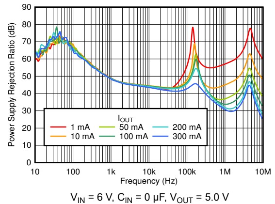
Figure 6-70. PSRR vs Frequency and I_{OUT}
