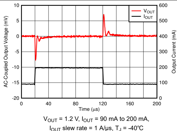
Figure 6-54. Load Transient
