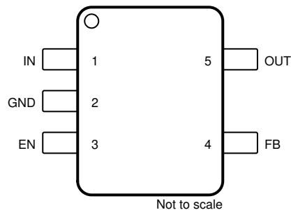
Figure 5-2. DBV Package (Adjustable), 5-Pin SOT-23, Top View
