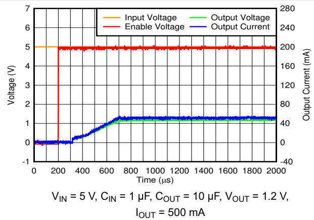
Figure 6-80. Start Up at 150^\circ\text{C}
