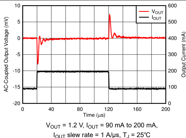
Figure 6-53. Load Transient
