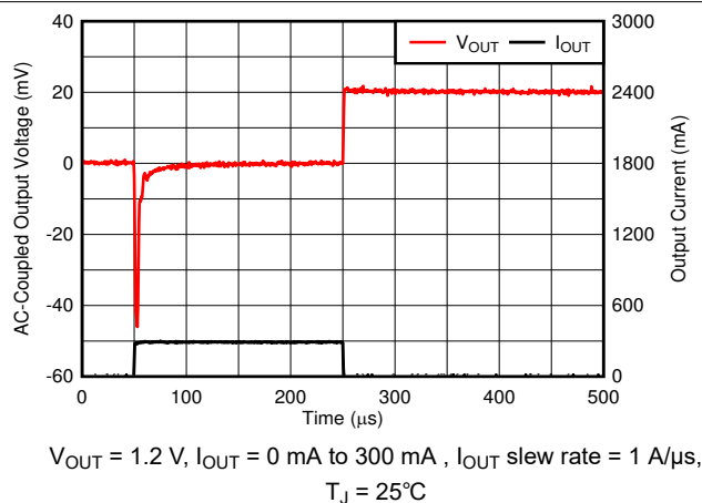
Figure 6-50. Load Transient
