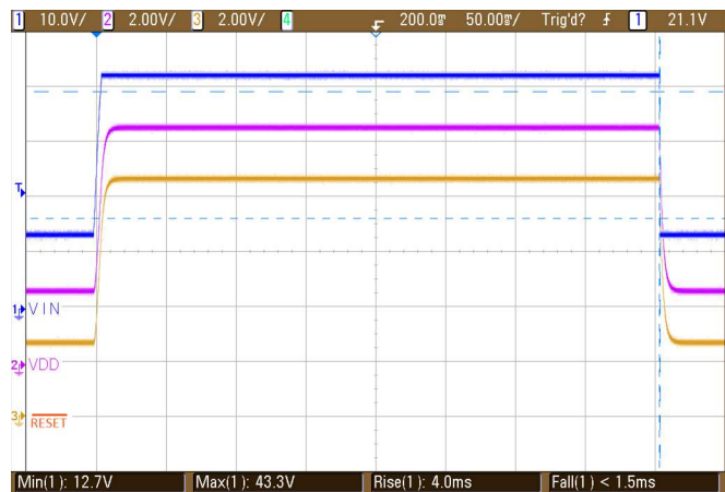
Figure 52. TPS3840-Q1 Cold-Start Test Pulse
