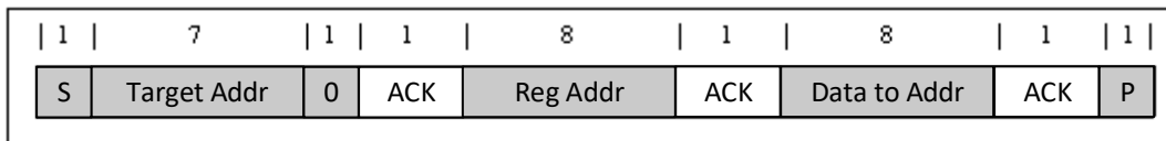
Figure 7-13. Single Write
