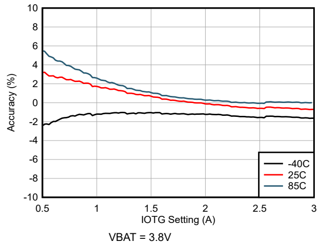
Figure 6-8. Boost Mode Current Limit Accuracy vs IOTG I²C Setting
