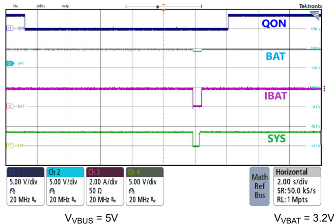
Figure 9-14. System Reset by QON With VBUS Present
