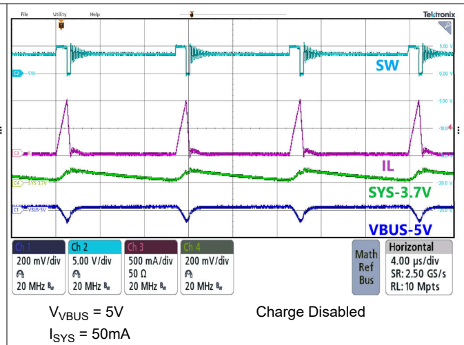
Figure 9-3. PFM Switching in Buck Mode
