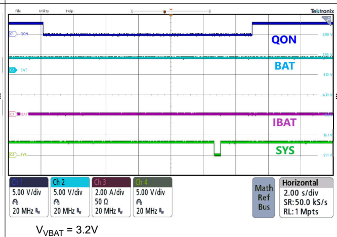
Figure 9-13. System Reset by QON Without VBUS Present
