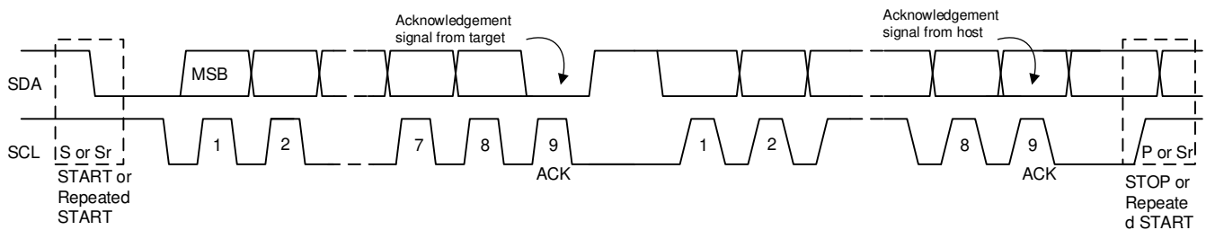
Figure 7-11. Data Transfer on the I²C Bus
