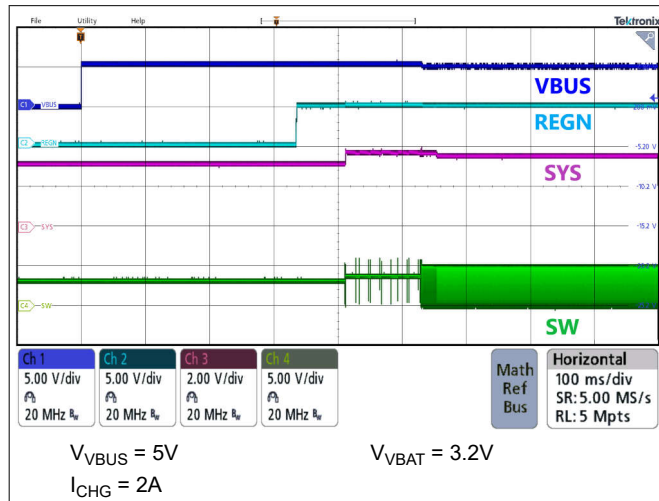
Figure 9-2. Power-Up With Charge Enabled
