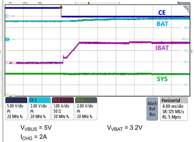
Figure 9-5. Charge Enable
