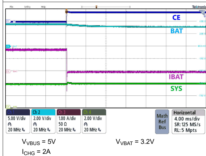
Figure 9-6. Charge Disable
