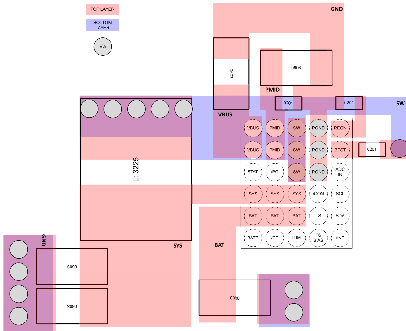
Figure 9-16. Layout Example
