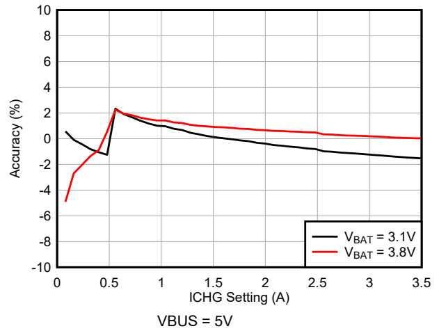
Figure 6-6. Charge Current Accuracy vs Charge Current I²C Setting
