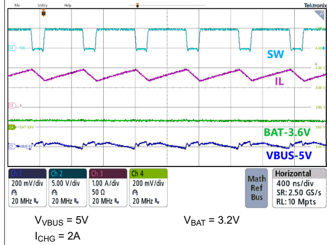
Figure 9-4. PWM Switching in Buck Mode
