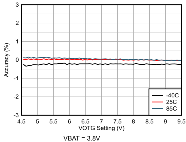
Figure 6-7. Boost Mode Voltage Accuracy vs VOTG I²C Setting
