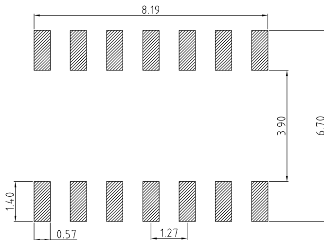
Figure 20. SO-14 recommended footprint
