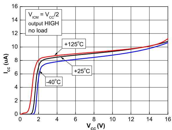
Figure 3. Current consumption vs. supply voltage, output high
