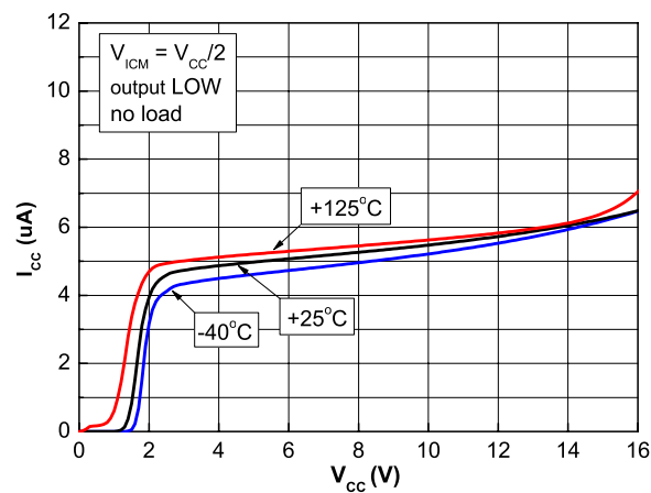
Figure 4. Current consumption vs. supply voltage, output low
