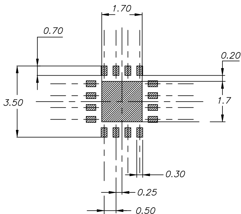
Figure 24. QFN16 3x3 recommended footprint
