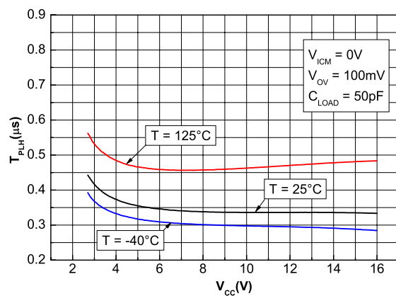
Figure 15. Propagation delay t_{PLH} vs. supply voltage
