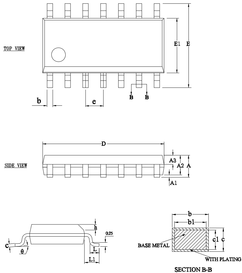
Figure 19. SO-14 package outline
