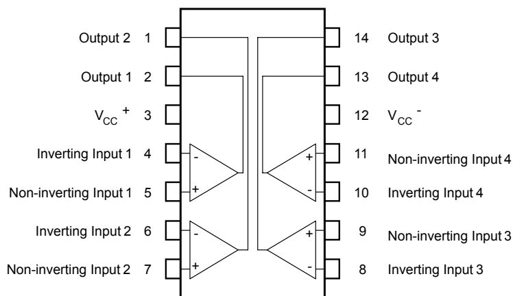
SO14 and TSSOP14
