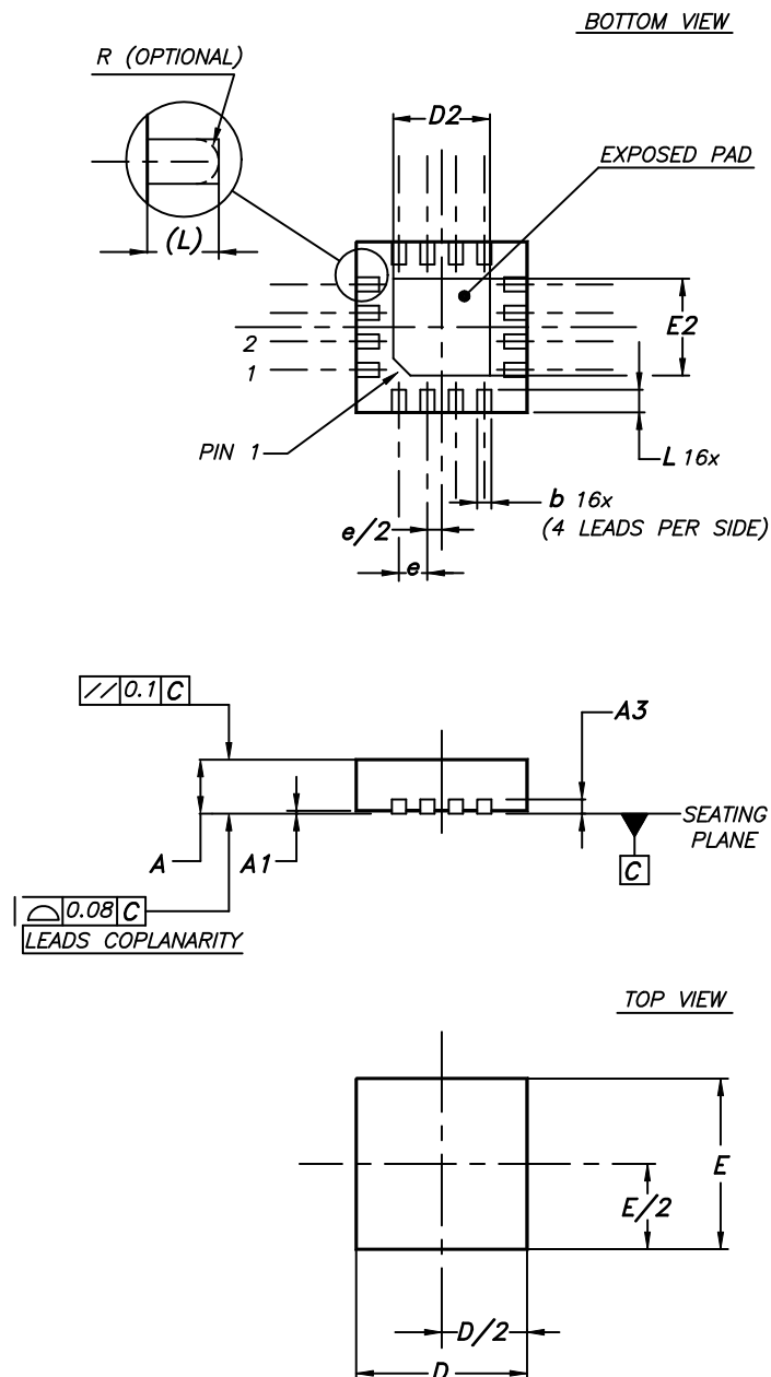
Figure 23. QFN16 3x3 package outline
