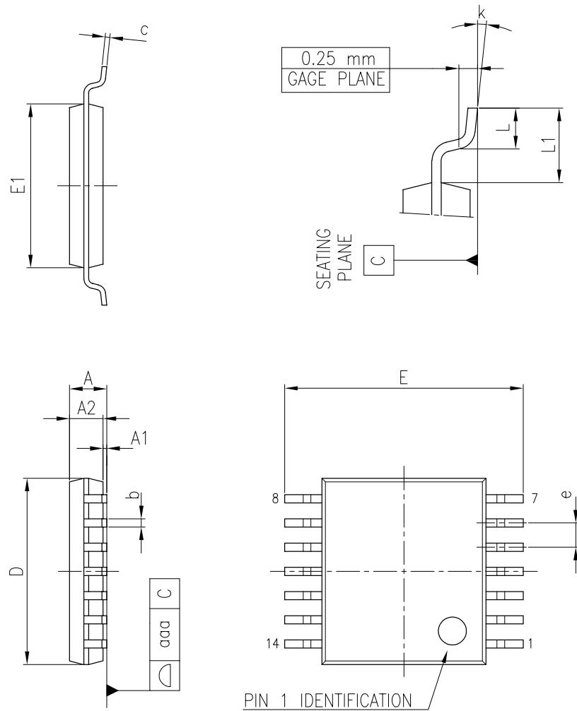
Figure 21. TSSOP-14 package outline
