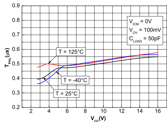
Figure 16. Propagation delay t_{PHL} vs. supply voltage
