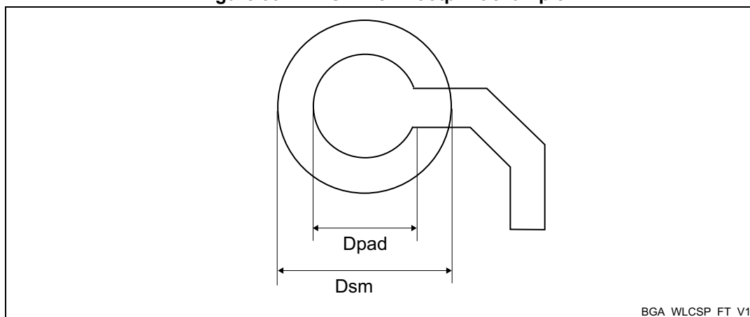
Figure 99. TFBGA225 - Footprint example
