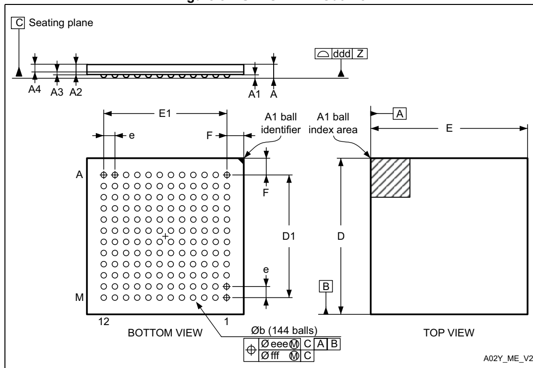
Figure 87. UFBGA144 - Outline
