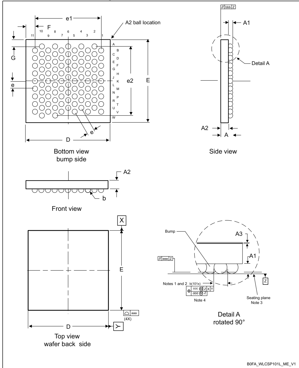
Figure 93. WLCSP101L - Outline
