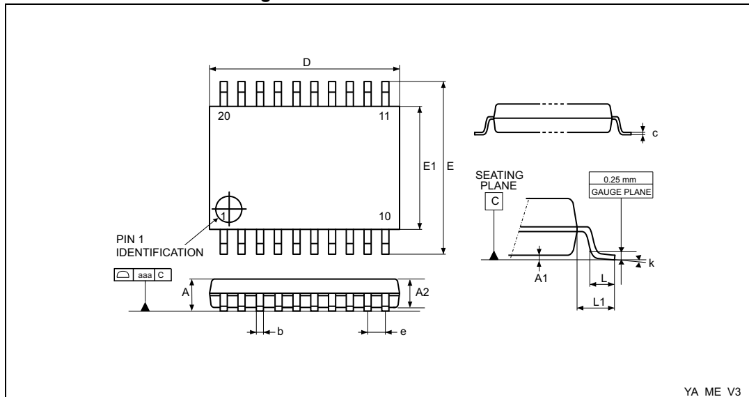
Figure 34. TSSOP20 – Outline
