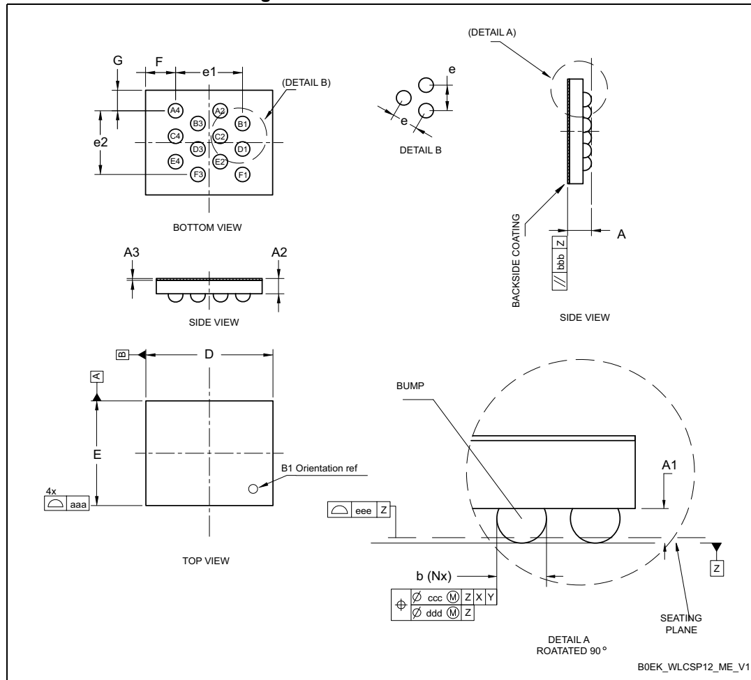
Figure 31. WLCSP12 – Outline
