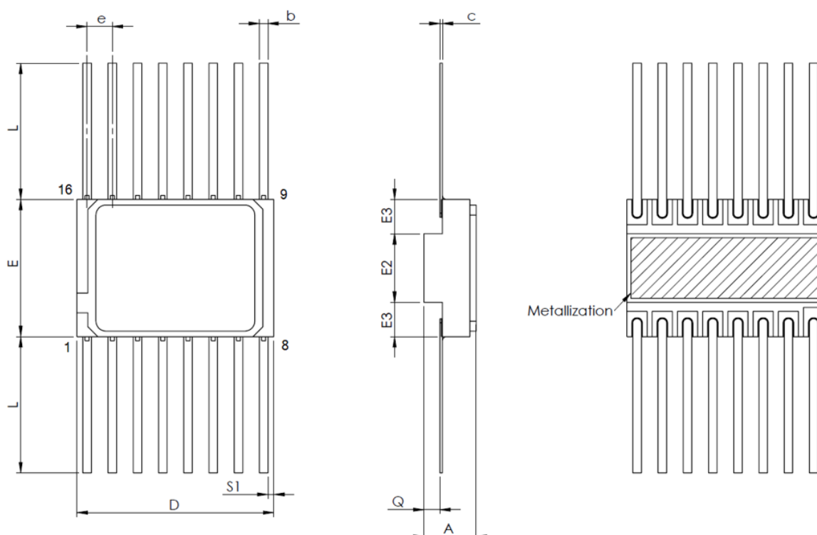
Figure 27. Flat-16P package outline
