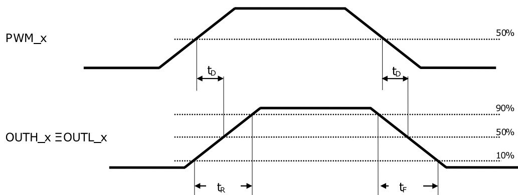
Figure 5. Time diagram
