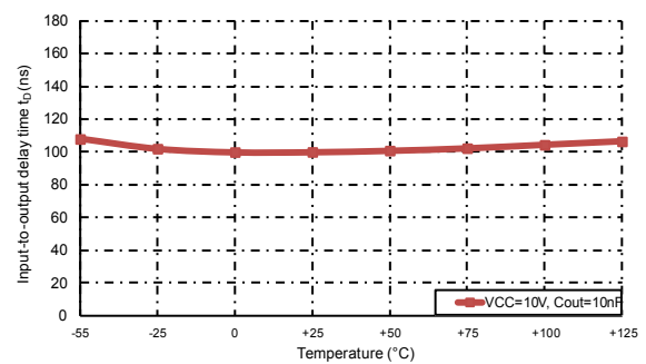
Figure 19. Input-to-output delay time vs temperature
