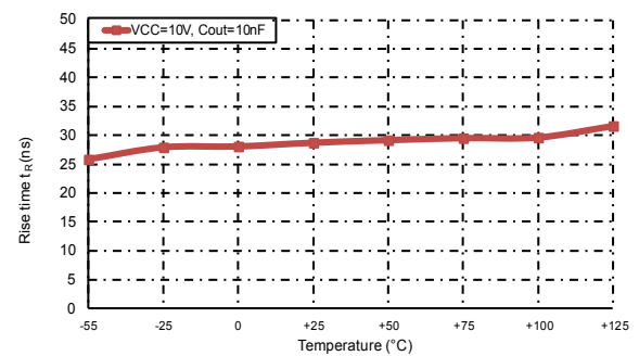
Figure 15. PWM_x rise time vs temperature
