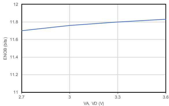
Figure 18. ENOB vs. power supply
