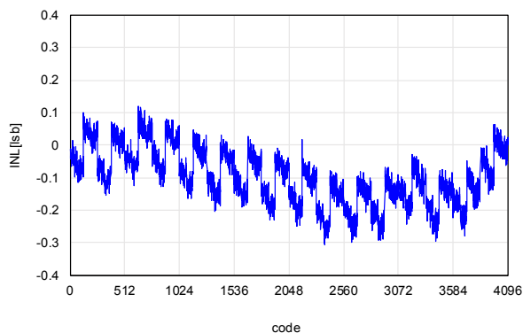
Figure 9. INL vs. output code @ V_A = V_D = 3.3 \text{ V}
