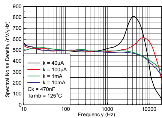
Figure 22. Spectral noise density vs. freq. at 125 °C, C_k = 470 \text{ nF}
