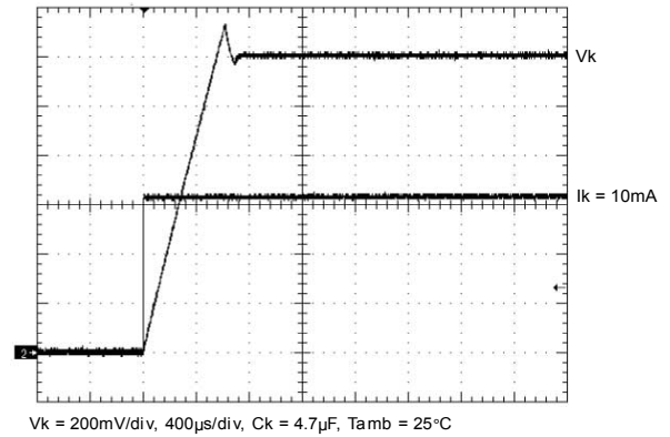
Figure 44. Cathode current step resp. at 25 °C, C_k = 4.7 µF, \Delta I_k = 10 mA
