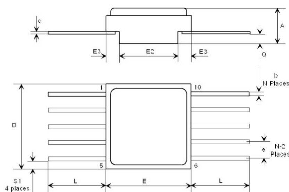
Figure 65. Ceramic Flat-10 package mechanical drawing
