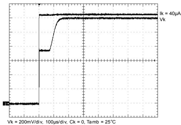
Figure 23. Cathode current step resp. at 25 °C, C_k = 0 , \Delta I_k = 40 \mu\text{A}
