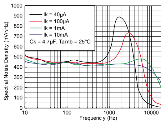
Figure 63. Spectral noise density vs. frequency
