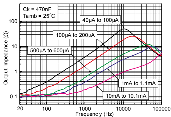
Figure 11. Output impedance vs. freq. at 25 °C, C_k = 470 nF
