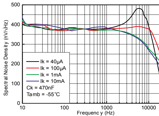
Figure 21. Spectral noise density vs. freq. at -55 °C, C_k = 470 \text{ nF}
