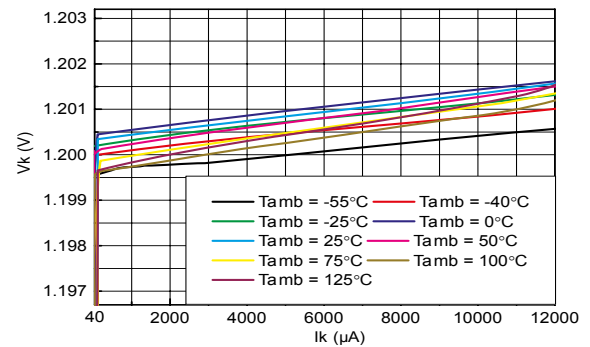
Figure 2. Zoom of reverse breakdown voltage characteristic vs. cathode current
