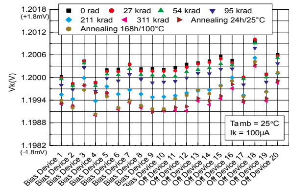
Figure 60. Reverse breakdown voltage vs. cumulated radiation dose (0.01 rad/s)
