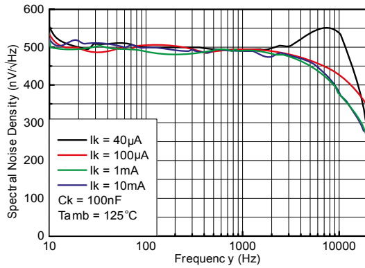
Figure 19. Spectral noise density vs. freq. at 125 °C, C_k = 100 \text{ nF}
