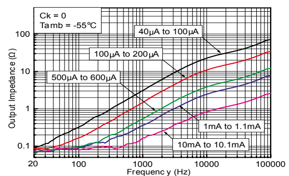
Figure 6. Output impedance vs. freq. at -55 °C, C k = 0
