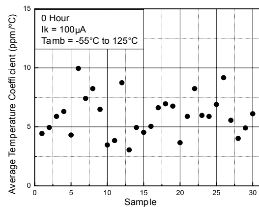
Figure 52. Average temperature coefficient at 0 hr, I k = 100 µA
