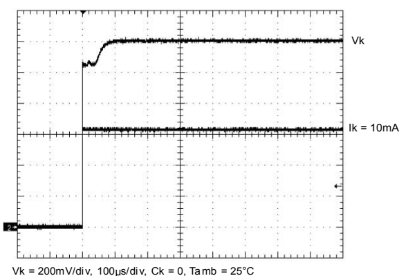
Figure 41. Cathode current step resp. at 25 °C, C_k = 0 , \Delta I_k = 10 mA
