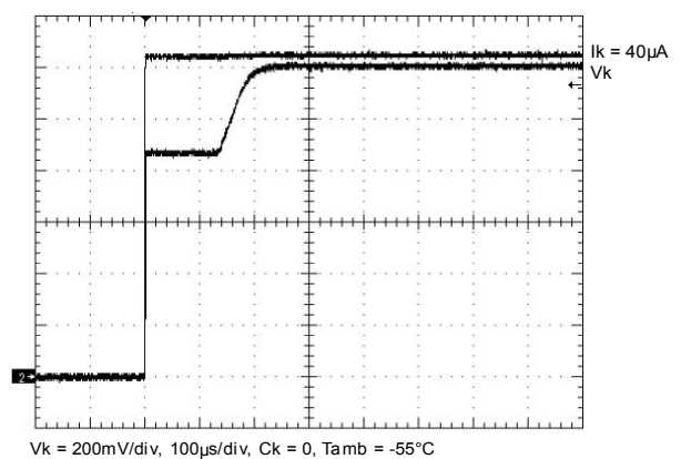
Figure 24. Cathode current step resp. at -55 °C, C_k = 0 , \Delta I_k = 40 \mu\text{A}
