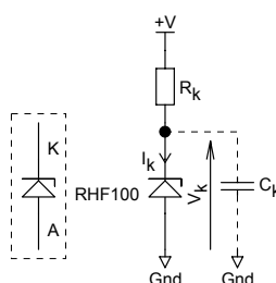
Figure 62. Implementation used for the test and for the characterisation
