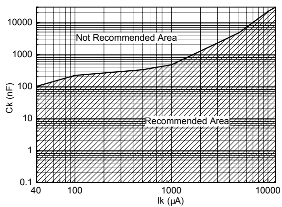
Figure 61. Recommended operating area
