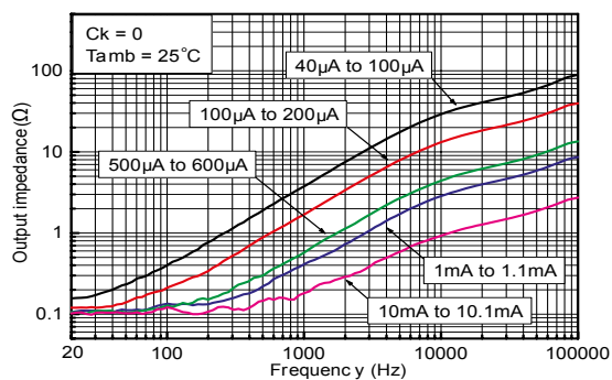
Figure 5. Output impedance vs. freq. at 25 °C, C k = 0
