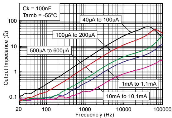
Figure 9. Output impedance vs. freq. at -55 °C, C_k = 100 nF
