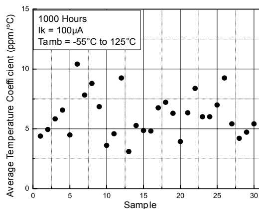
Figure 53. Average temperature coefficient at 1000 hrs, I k = 100 µA
