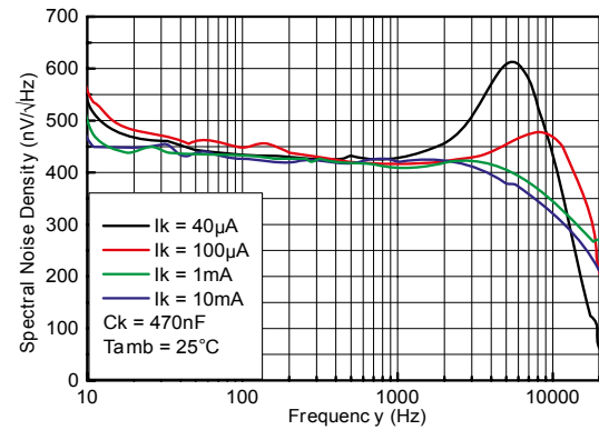
Figure 20. Spectral noise density vs. freq. at 25 °C, C_k = 470 \text{ nF}
