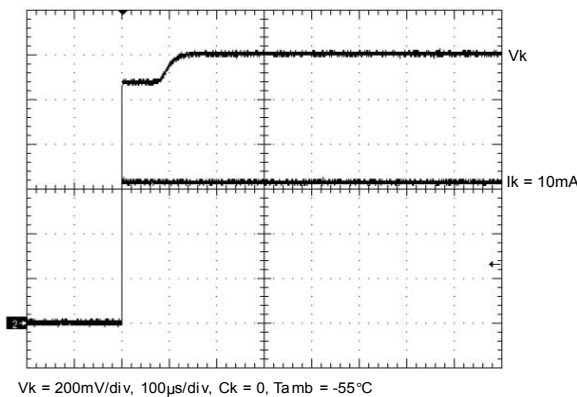
Figure 42. Cathode current step resp. at -55 °C, C_k = 0 , \Delta I_k = 10 mA
