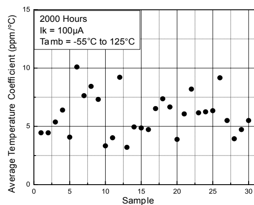
Figure 54. Average temperature coefficient at 2000 hrs, I k = 100 µA
