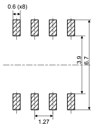
Figure 33. SO8N - Footprint example
