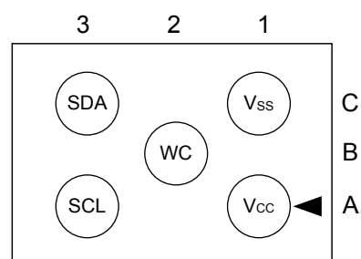
Bump side (bottom view)
