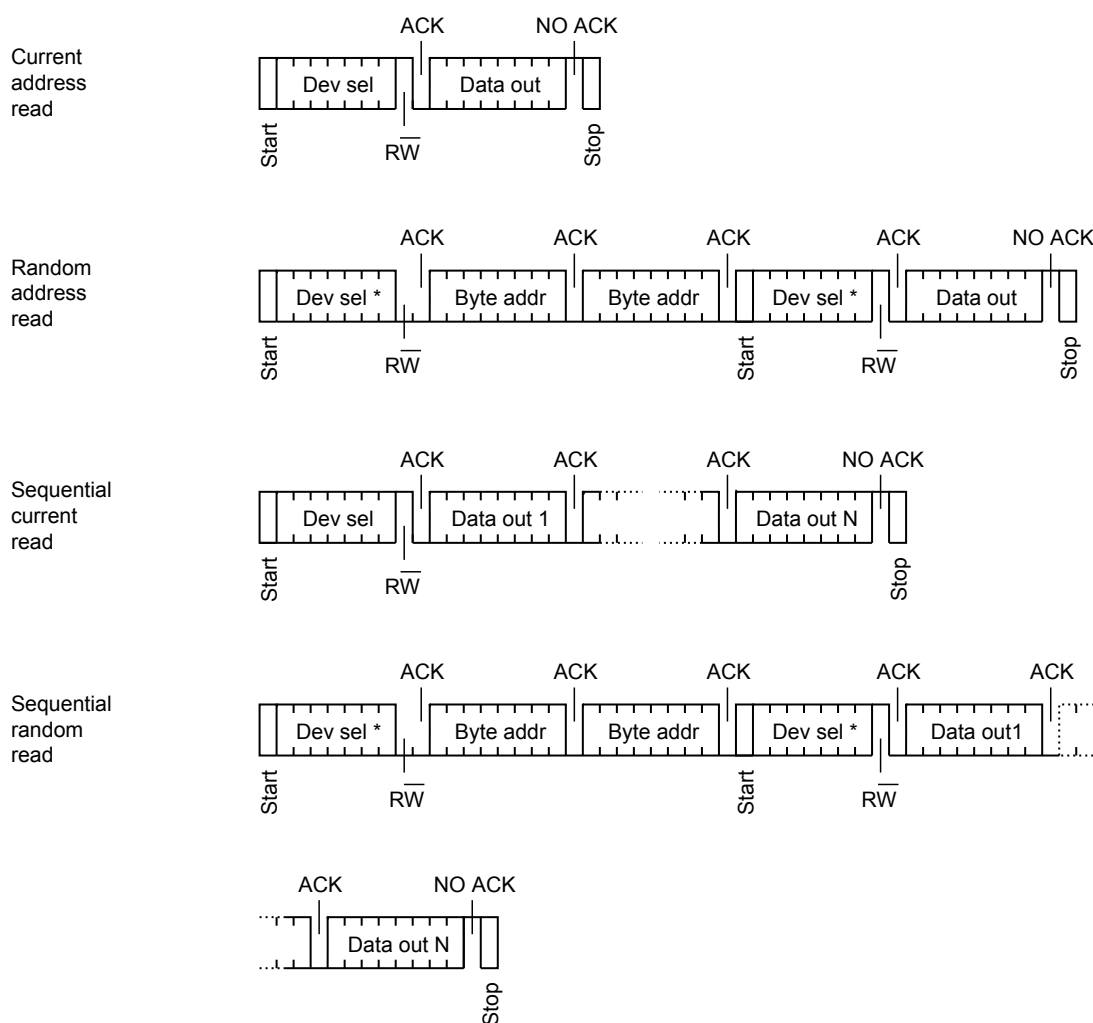
Figure 17. Read mode sequences
