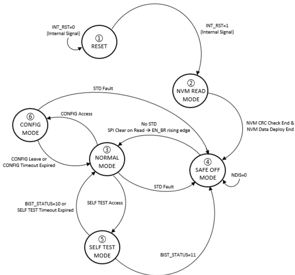
Figure 11. Device operational state machine
