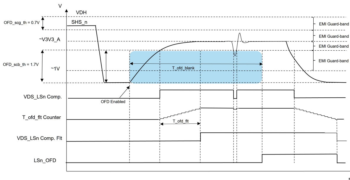
Figure 68. OFD masking and deglitch filtering - LSn_OFD example
