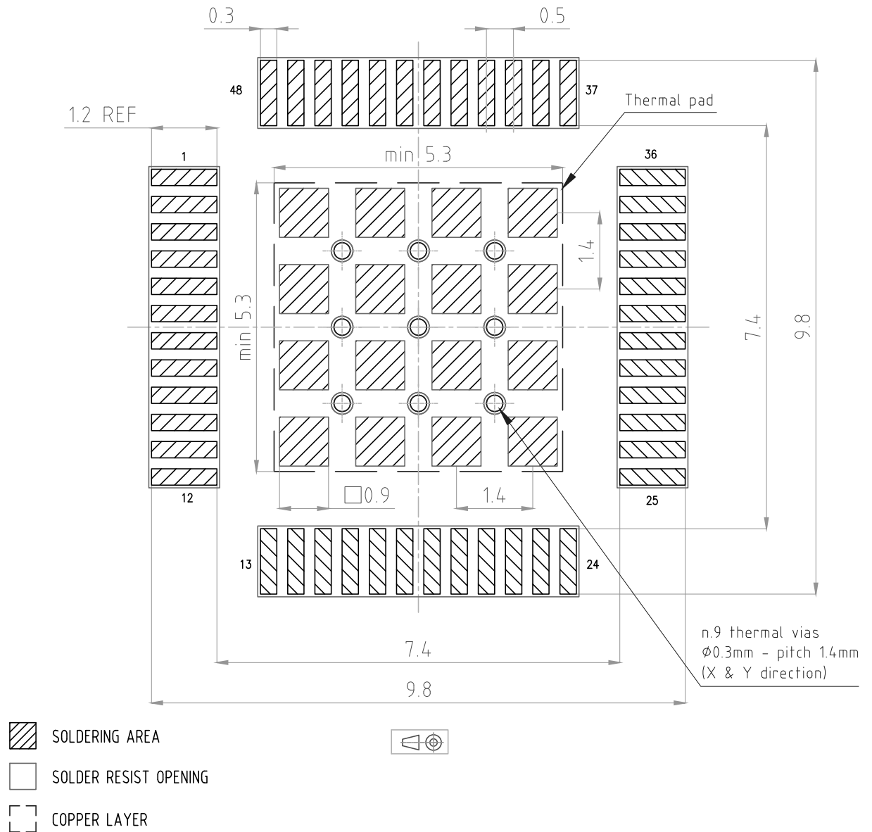
Figure 93. Suggested PCB landpattern
