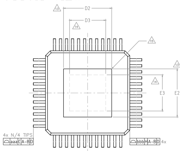
Figure 92. TQFP48 (7x7x1 mm exp. pad down) package outline
