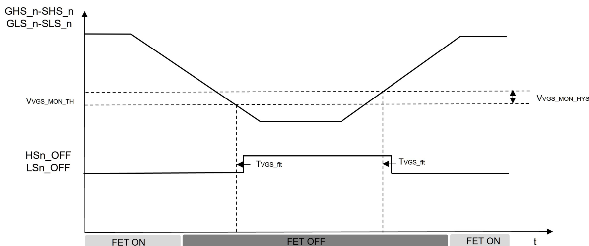
Figure 39. VGS monitor operative ranges
