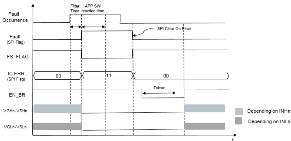
Figure 16. Shutdown fault - Permanent fault timing diagram
