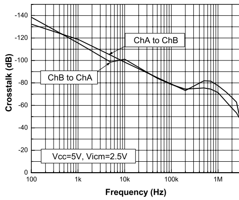
Figure 44. Crosstalk vs. frequency
