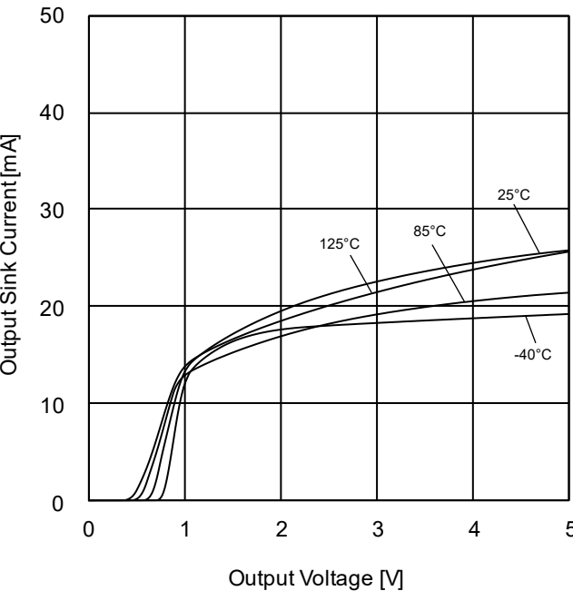
Figure 37. Output Sink Current vs Output Voltage ( V_{CC}=5V )
