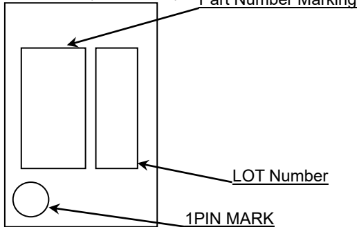
TSSOP-B8(TOP VIEW)
