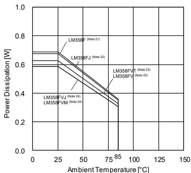
(c) LM358xxx
