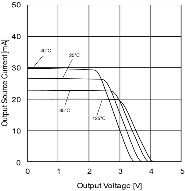
Figure 35. Output Source Current vs Output Voltage ( V_{CC}=5V )
