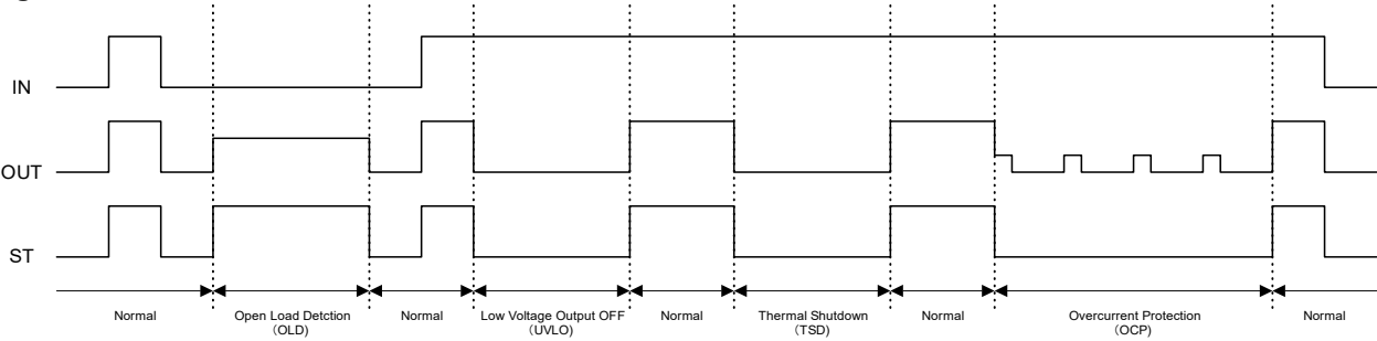
Figure 45. Timing Chart
