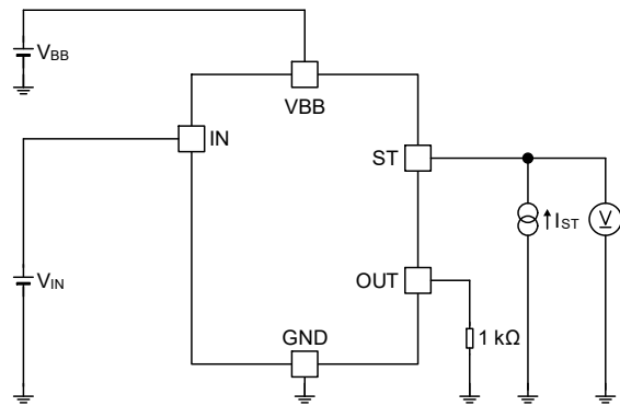
Figure 41. Diagnostic Output Low Voltage
