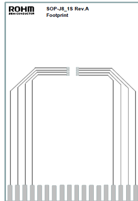
Figure 6. PCB Layout 1 layer (1s)
