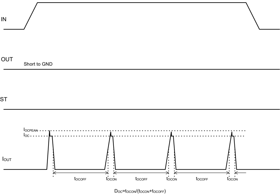
Figure 44. Overcurrent Detection Current Overcurrent Detection Peak Current Overcurrent Detection ON Time Overcurrent Detection OFF Time Overcurrent Detection ON Duty
