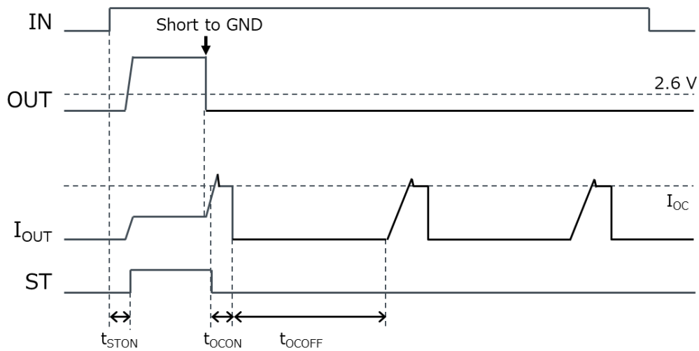
Figure 46. Overcurrent Protection Timing Chart (Short to GND)
