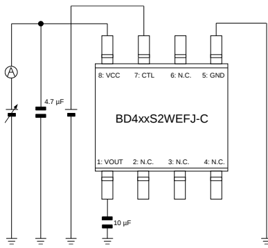
Measurement Setup for Figure 5, 7, 16, 17, 21, Figure 23, 25, 34, 35, 39
