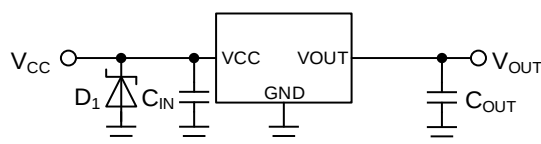
Figure 44. Surges Higher than absolute maximum ratings are Applied to the Input
