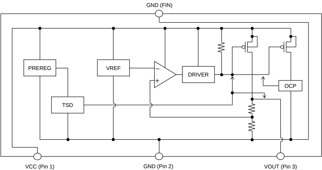
Figure 4. Block Diagrams
