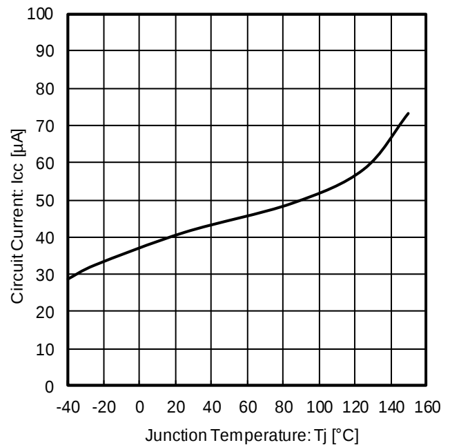
Figure 34. Circuit Current vs Temperature
