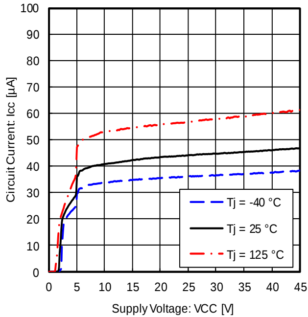
Figure 23. Circuit Current vs Power Supply Voltage
