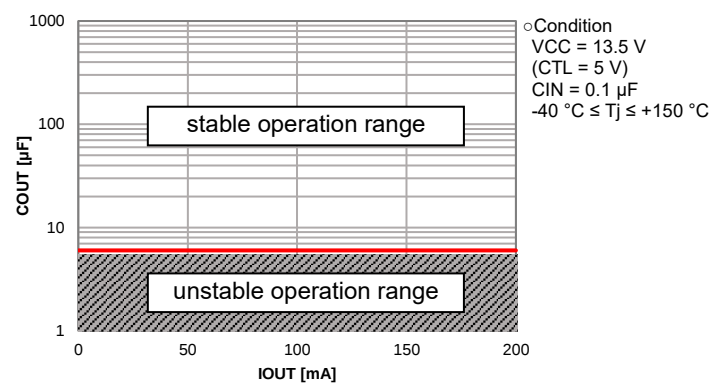
Figure 42. COUT (Typ) vs IOUT
