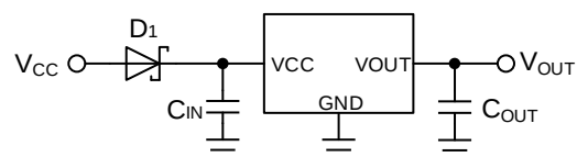
Figure 50. Protection against Reverse Polarity 1
