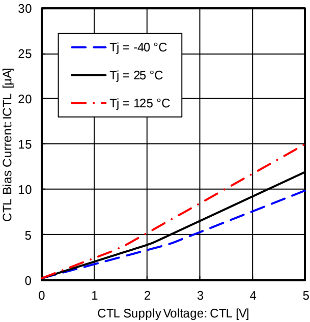
Figure 40. CTL Bias Current vs CTL Supply Voltage
