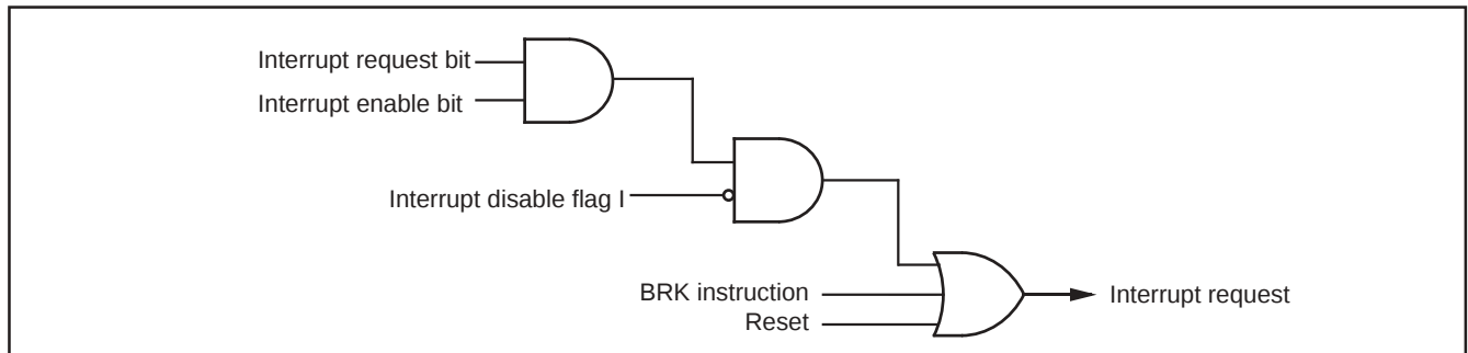
Fig. 19 Interrupt control
