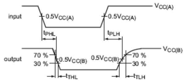
Figure 13. Propagation Delay and Transition Times; Port A to Port B
