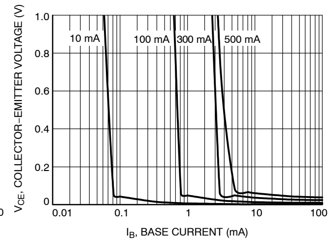
Figure 20. Saturation Region
