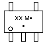
SC-88A CASE 419A
