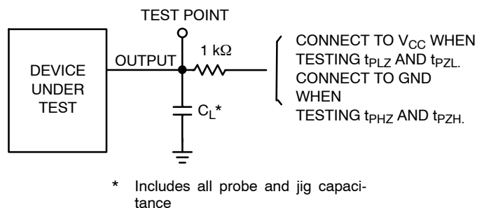
Figure 6. Test Circuit
