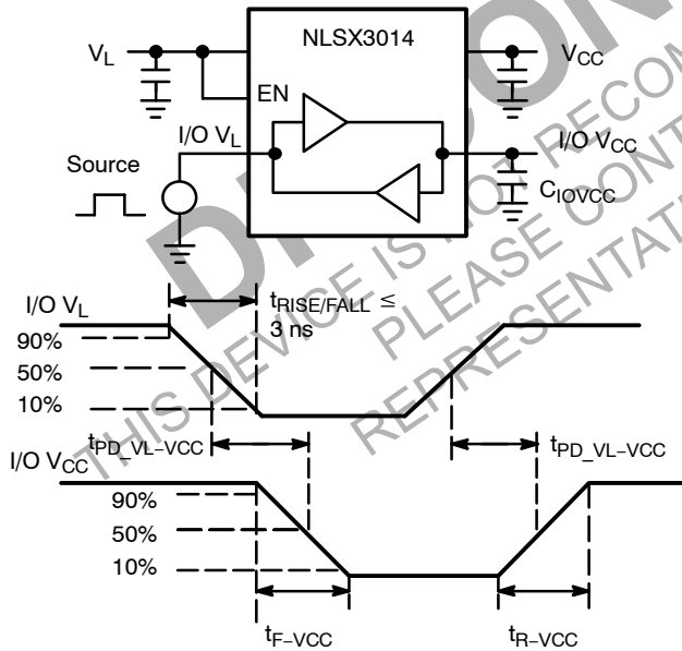
Figure 3. Driving I/O V_L Test Circuit and Timing
