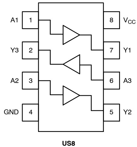
Figure 2. Pinout
