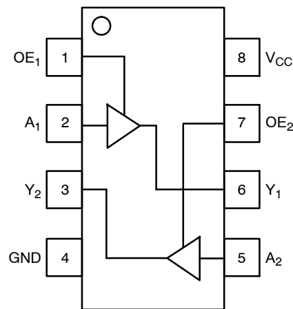
US8 Figure 2. Pinout
