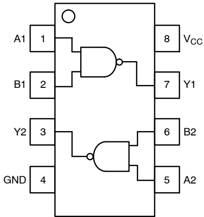
Figure 2. Pinout
