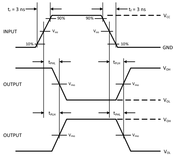
Figure 6. Switching Waveforms
