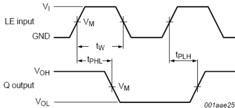
Figure 5. t_{PLH} , t_{PHL} , t_W Waveforms (LE to Q)
