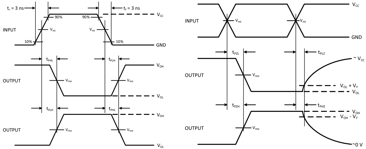
Figure 6. Switching Waveforms
