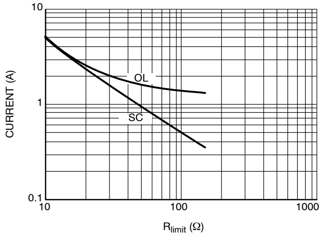
Figure 13. Current Limit vs. R_{\text{sense}} for Direct Current Sensing
