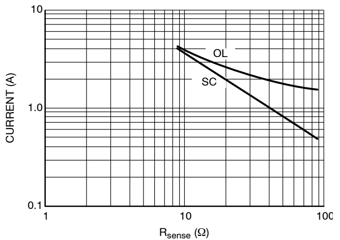
Figure 15. Current Limit vs. R_{\text{sense}} for Kelvin Current Sensing
