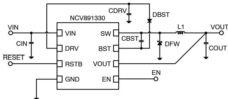
Figure 1. Typical Application
