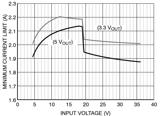
Figure 26. NCV890203 Load Current Capability with 4.7 \mu\text{H} Inductor
