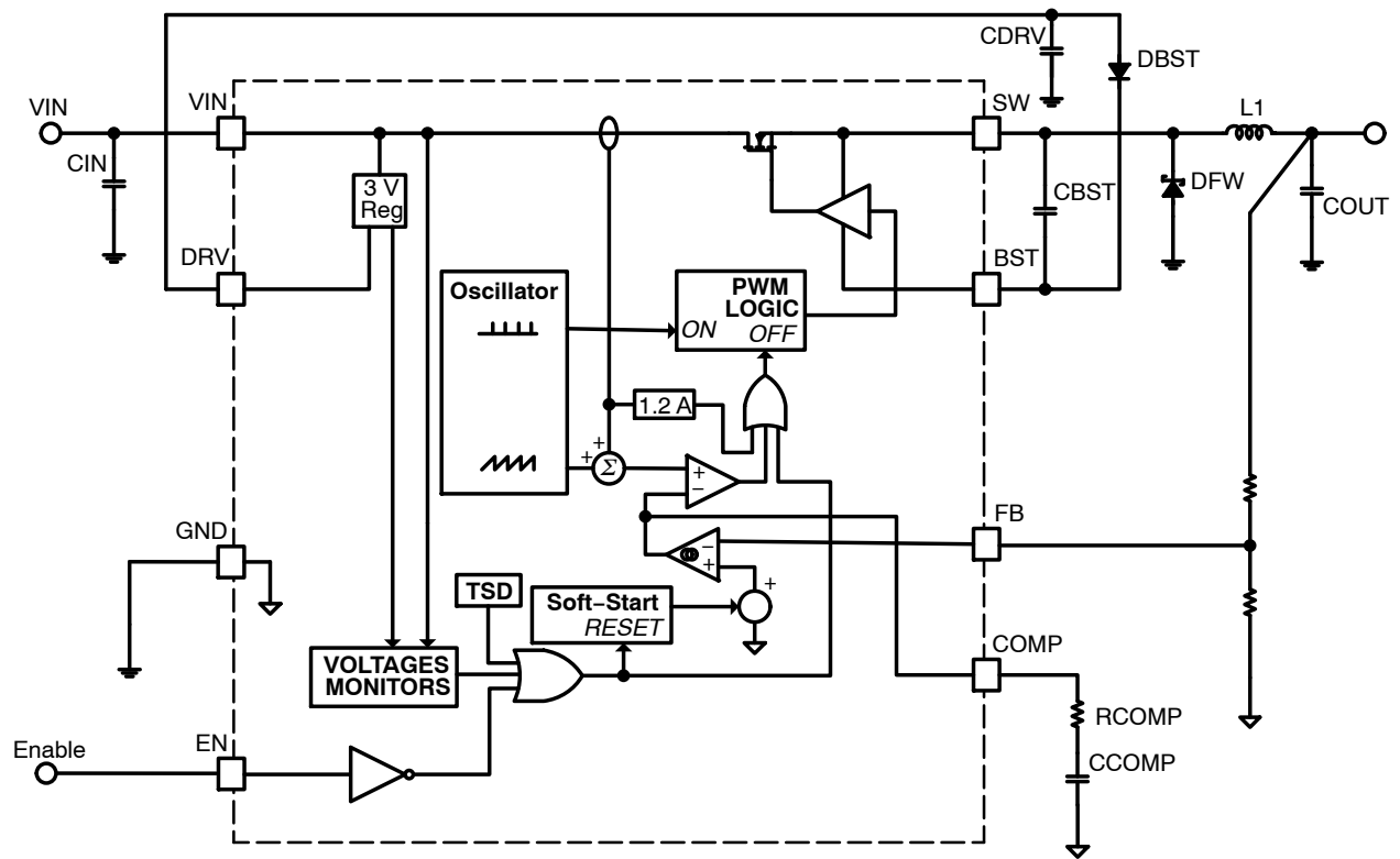
Figure 2. NCV890130 Block Diagram
