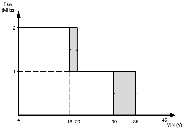
Figure 25. NCV890130 Switching Frequency Reduction at High Input Voltage
