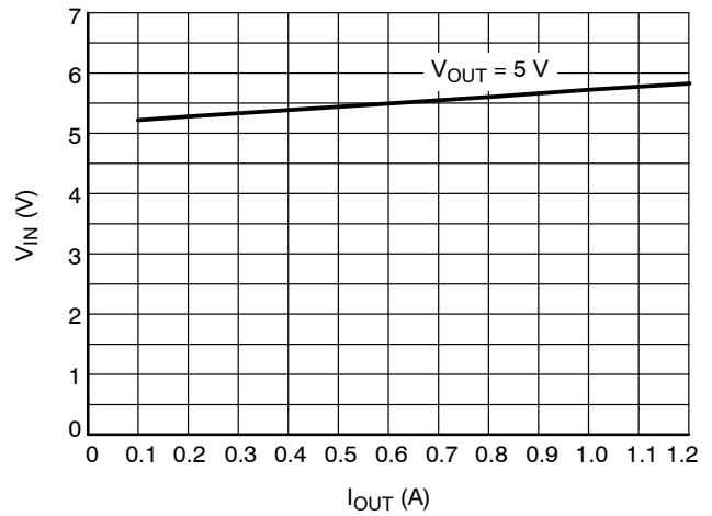
Figure 29. Minimum Input Voltage vs. Output Current
