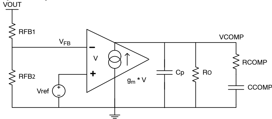
Figure 30. Feedback Compensator Network Model
