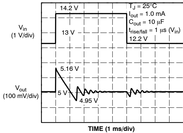
Figure 14. Line Transients
