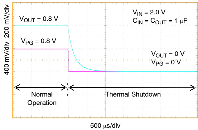
Figure 30. Turn-Off Response Due to Thermal Shutdown NCV8752A/B, V_{OUT} = 0.8\text{ V}
