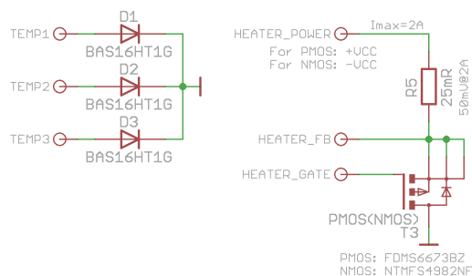
Figure 88. Thermal Circuit (All Demo Boards)
