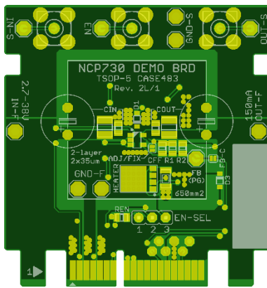
Figure 90. NCV8730 Demo Board (2 layer, rev. 1) – PCB Top Layer
