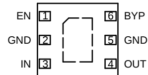
DFN6 (Top View)
