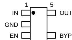
TSOP-5 (Top View)
