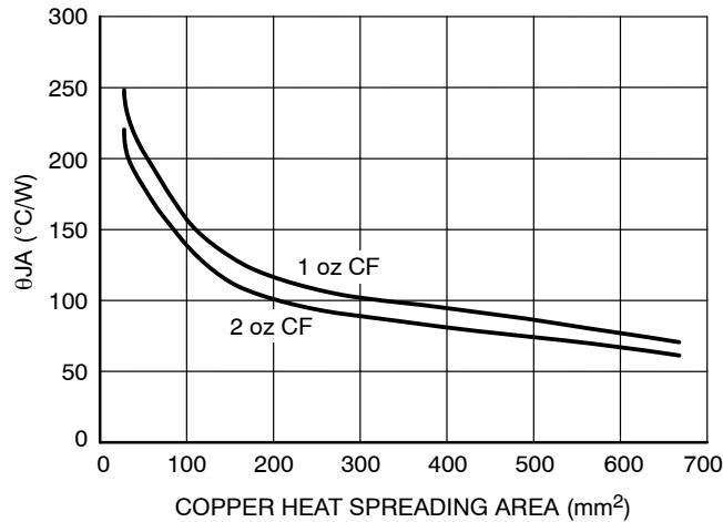
Figure 25. DFN 10 Self Heating Thermal Characteristic as a Function of Copper Area on the PCB
