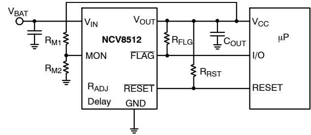
Figure 13. FLAG/Monitor Function
