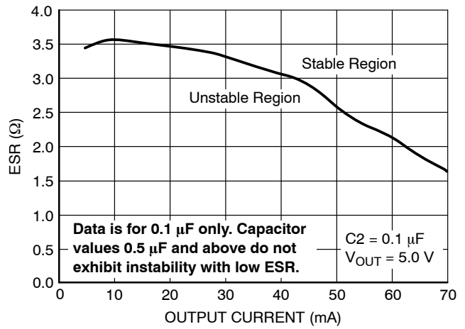
Figure 5. Output Stability with 0.1 \mu\text{F} at Low ESR
