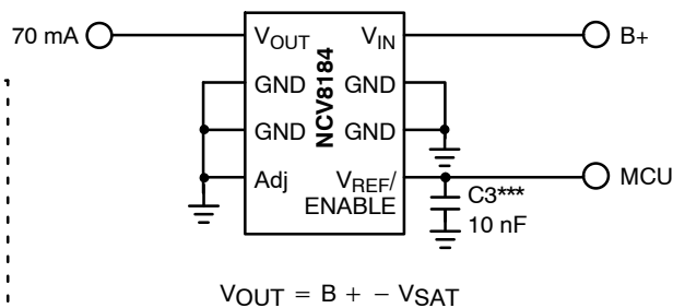
Figure 18. High-Side Driver
