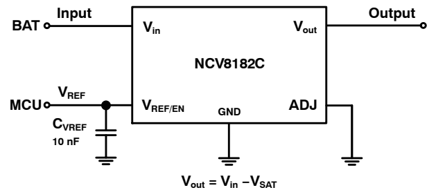
Figure 25. High-Side Driver
