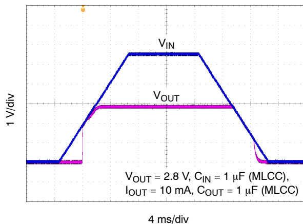
Figure 29. Turn-on/off – Slow Rising V_{IN}
