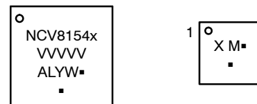
WDFN6 (Top View)
