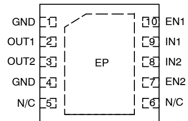
DFN10 (Top View)
