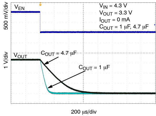
Figure 49. Enable Turn-off, V_{OUT} = 3.3 \text{ V}
