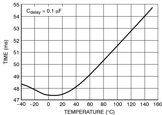
Figure 6. Delay Time
