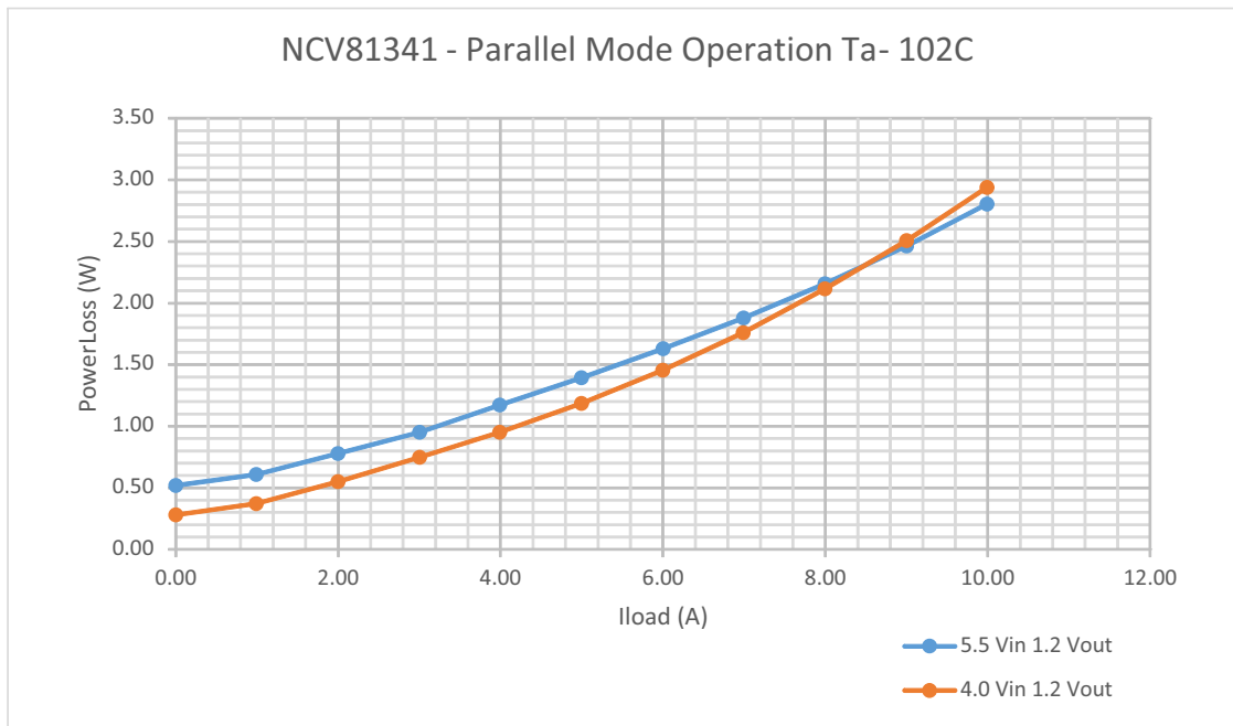
Figure 3. Power Loss vs Iload, T_A = 102\text{ }^{\circ}\text{C}
