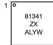
WQFNW20 3.5x3.5 CASE 512AB
