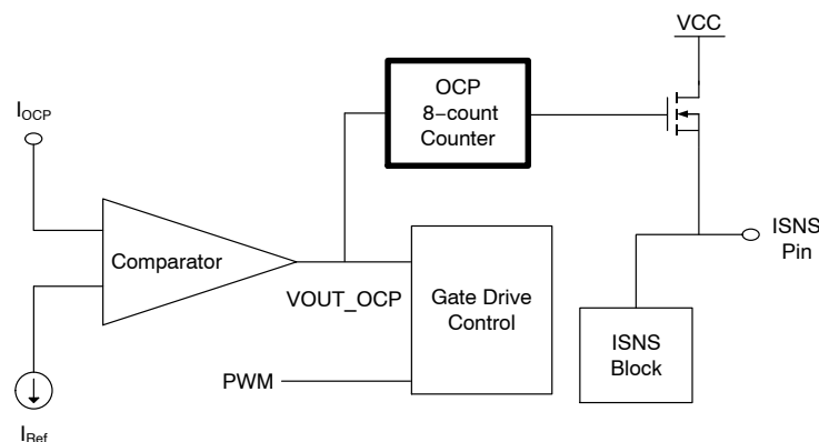
Figure 5. OCP Circuit Block Diagram
