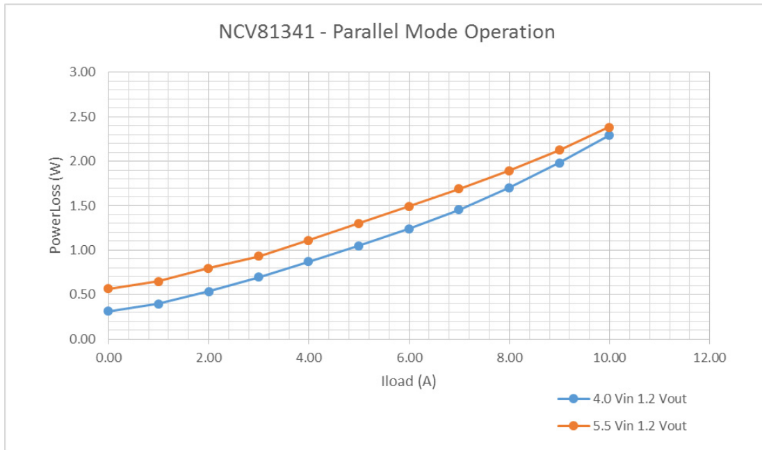
Figure 2. Power Loss vs Iload, T_A = 25\text{ }^{\circ}\text{C}
